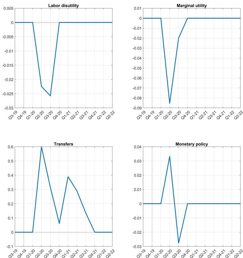
Figure 3: Time series estimated for COVID shocks, 2019Q3-2022Q2. The vertical dashed line corresponds to 2019Q4. See text for details.
