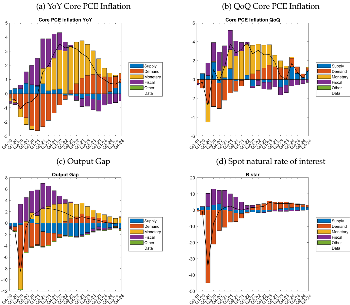
Figure 4: Simplified historical decompositions 2019Q4-2024Q4, relative to steady state value of the variable.
