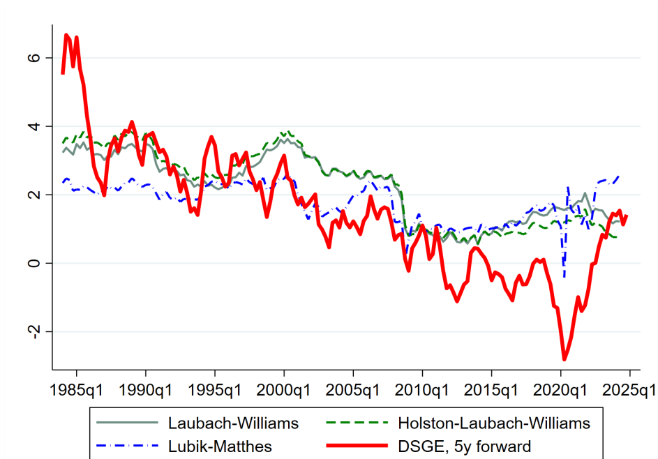
Figure 6: Standard measures of r^* versus model-implied \mathbb{E}_t r_{t+20}^f . Sources: FRB New York and FRB Richmond.
