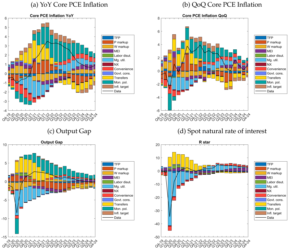
Figure 7: Detailed historical decompositions 2019Q4-2024Q4, relative to steady state value of the variable
